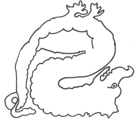
Draco Constellation - English
